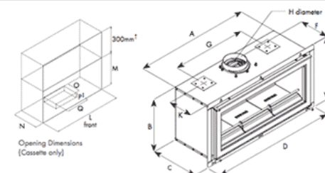
CASSETTE DIMENSIONS
