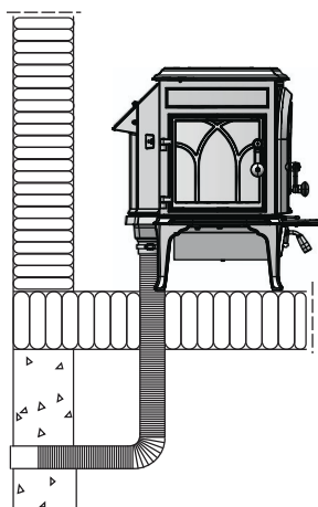
Fig. 9c Through the floor and basement
