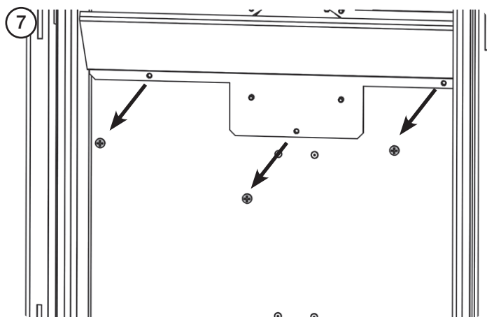
LOWER BAFFLE
