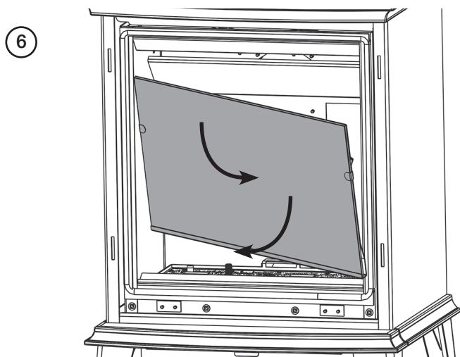
LOWER BAFFLE
