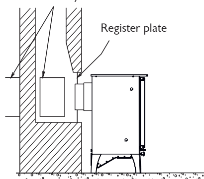
Fig. 6 Horizontal Register Plate With Rear Flue Connection
