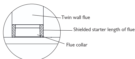
Fig. 3 Shielding the flue spigot
