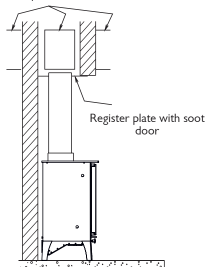
Fig. 7 Horizontal Register Plate With Top Flue Connection
